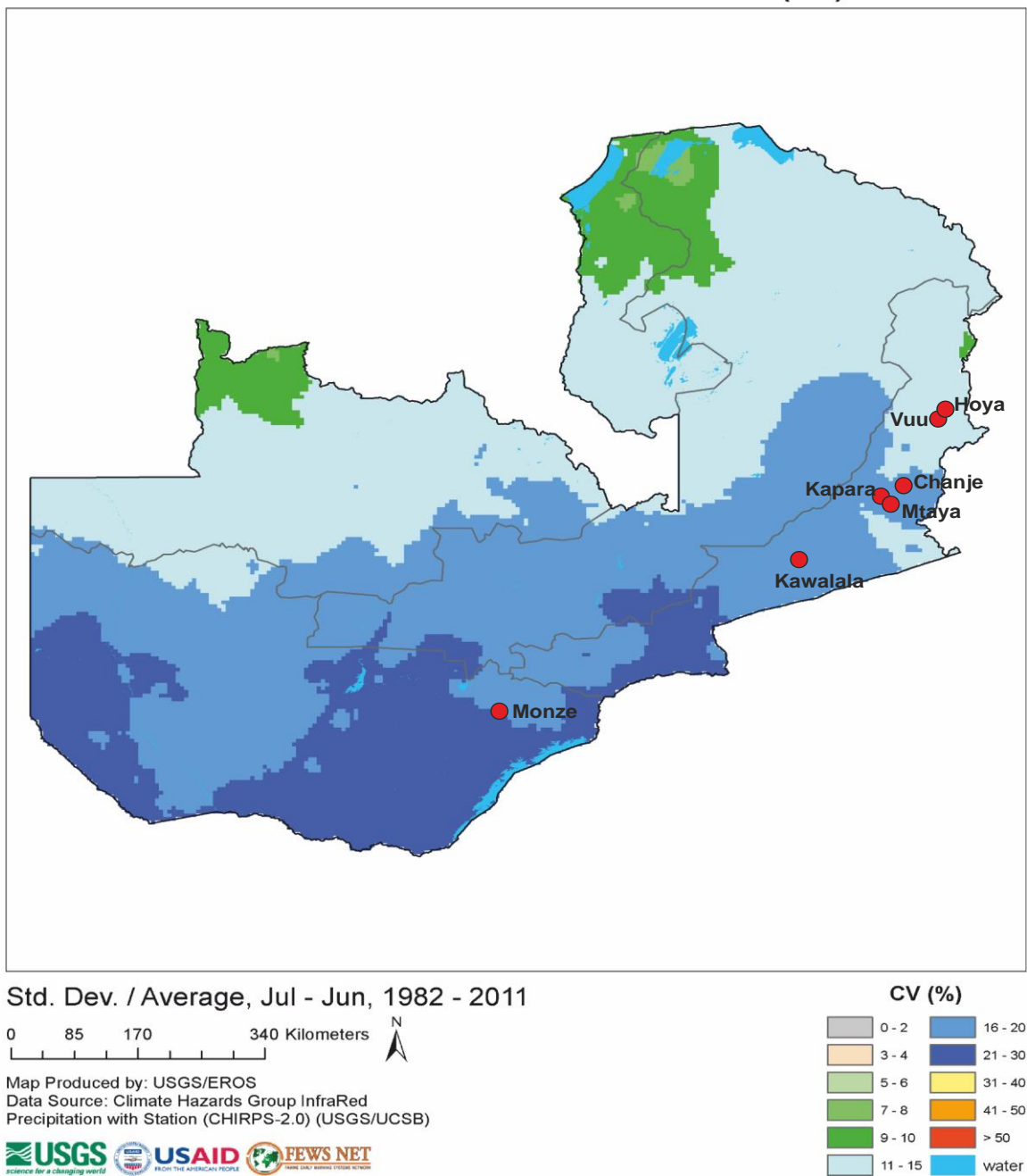
Figure 4: Zambia Rainfall coefficient variation 1982- 2011 source: southern Africa Famine Early Warning Systems Network, March 2018
